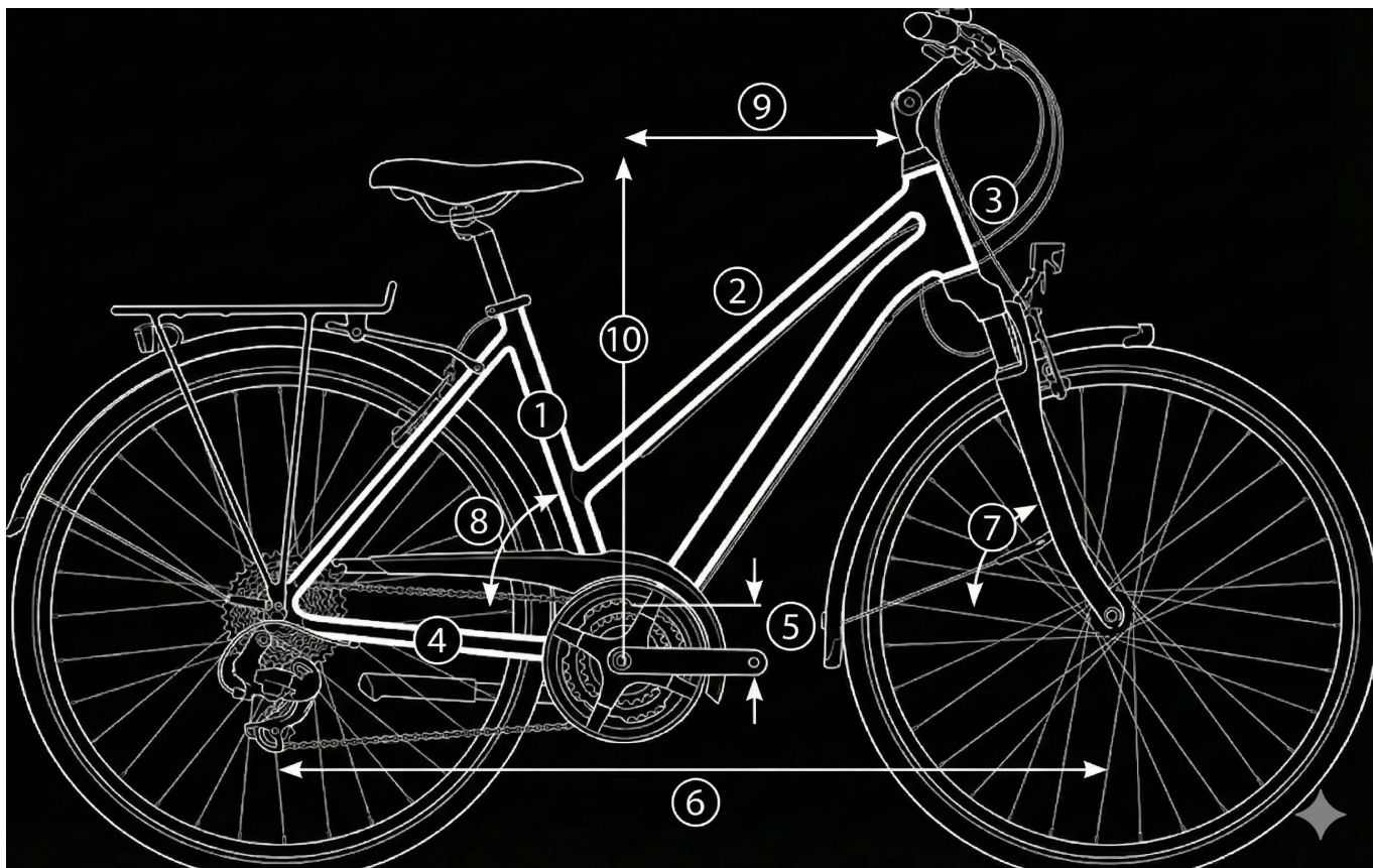
Schemat geometrii Winora Domingo X24 Mid
