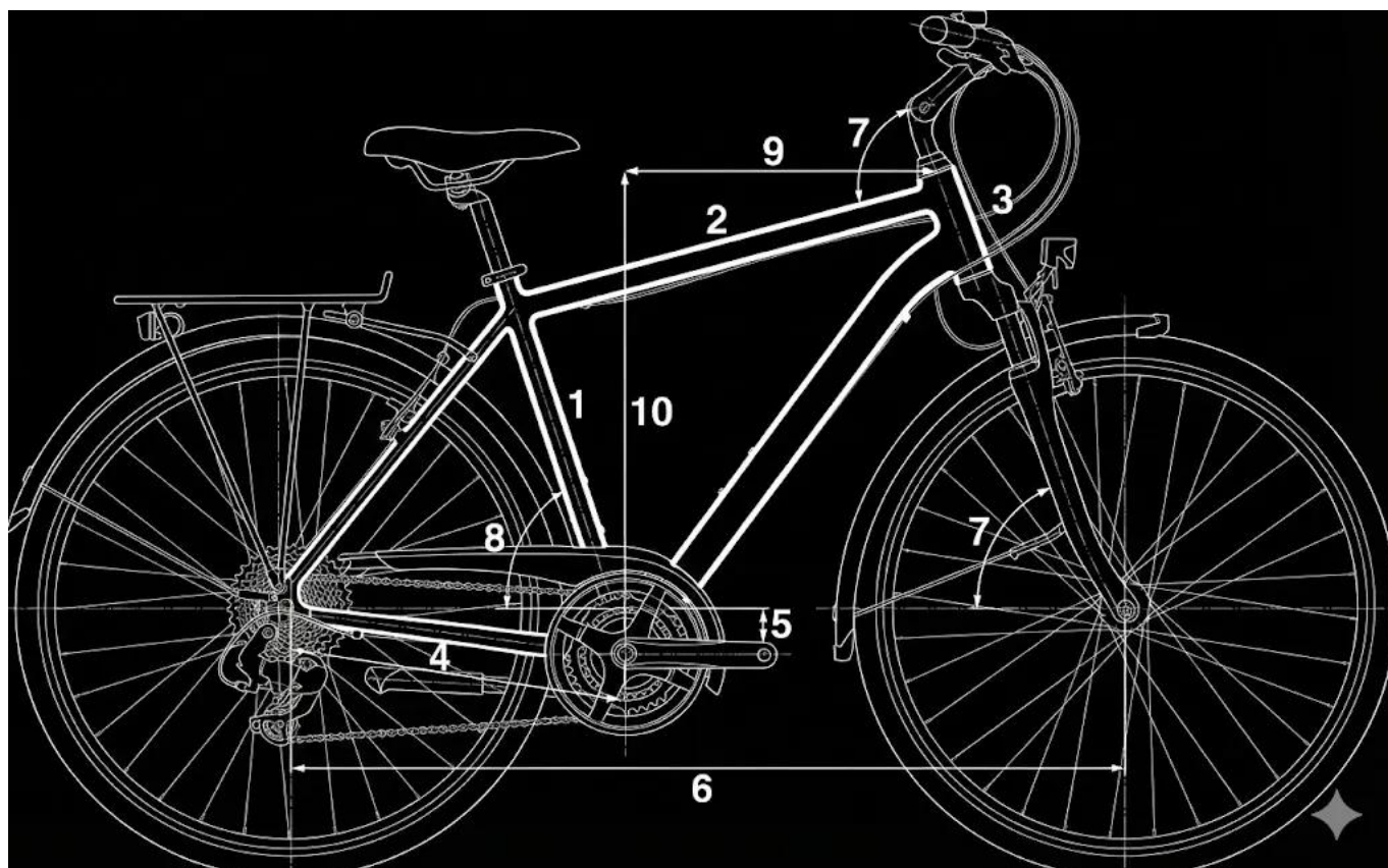
Schemat geometrii Winora Domingo X24 High
