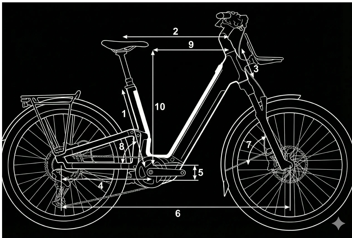
Winora Sinus FS ENV Low (Full Suspension)
