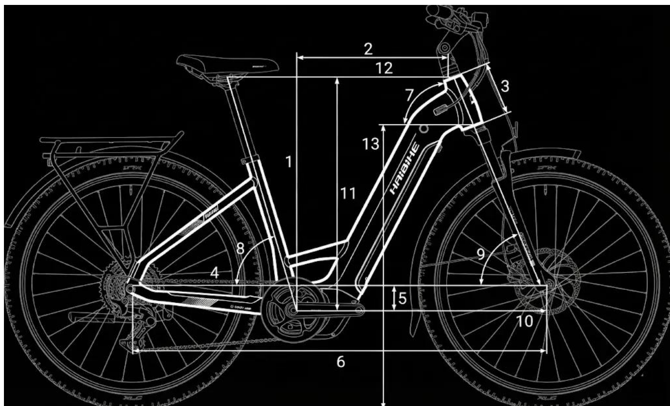
Geometria ramy Haibike TREKKING 7.5 Low
