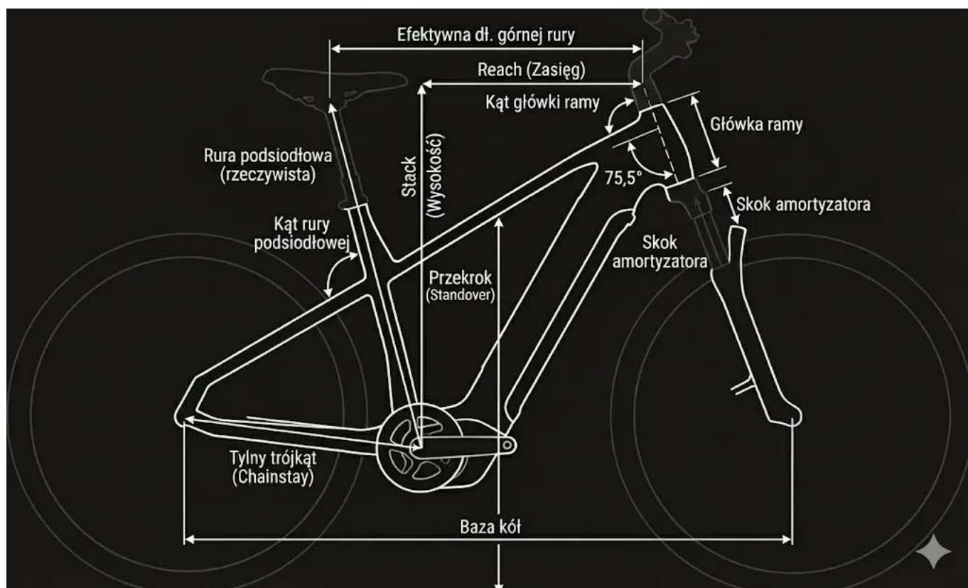
Geometria ramy Haibike TREKKING 7
