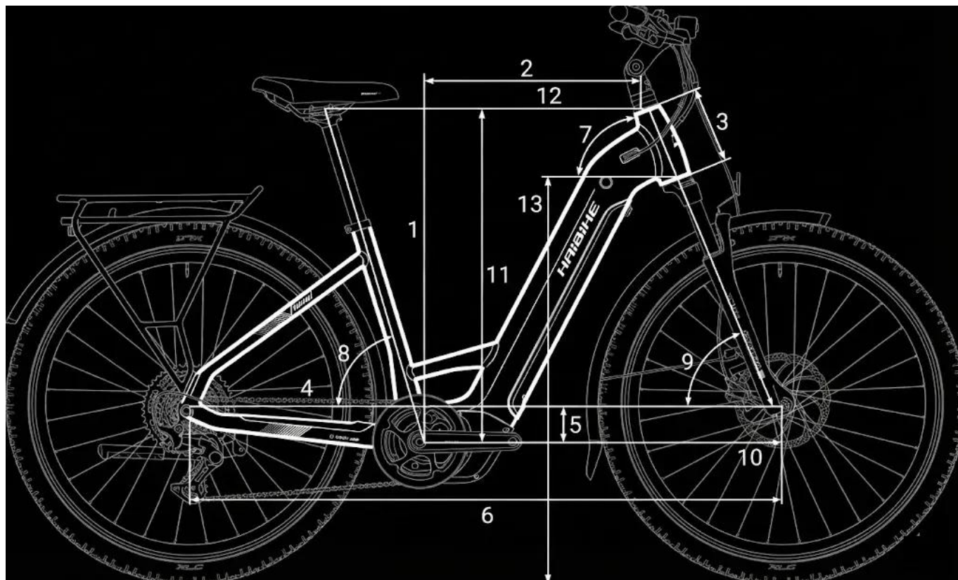
Geometria ramy Haibike TREKKING 3 Low
