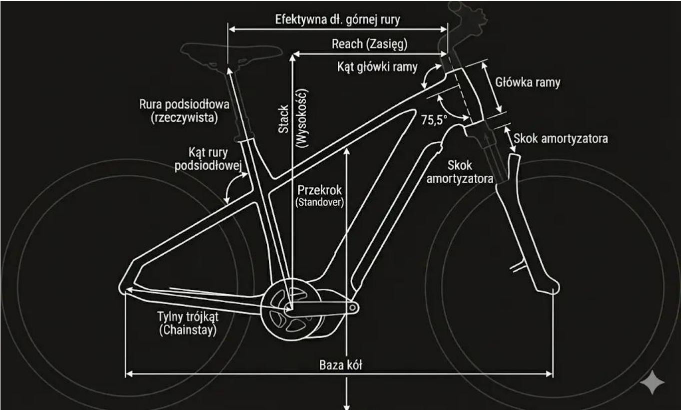
Geometria ramy Haibike TREKKING 3 High
