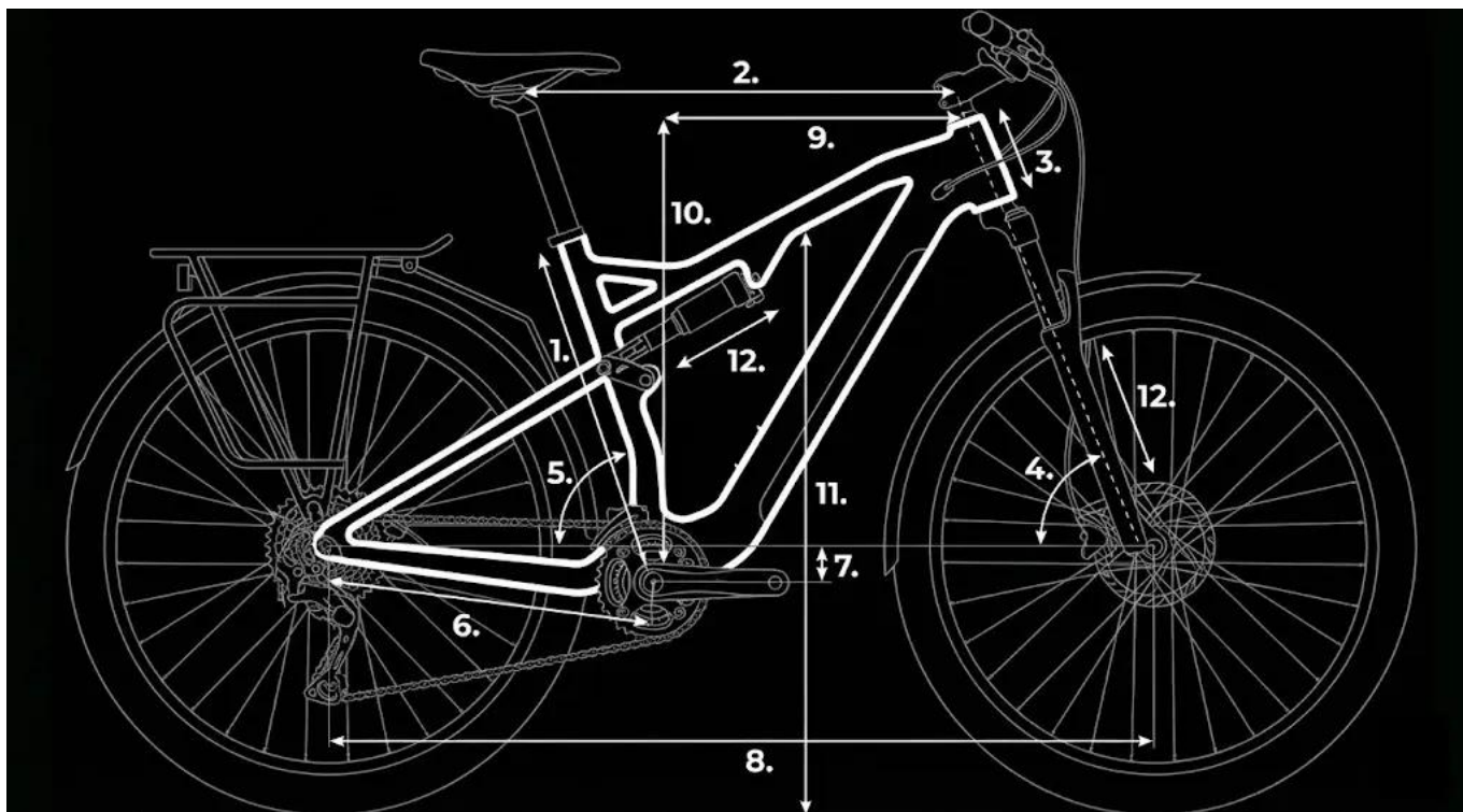
Geometria ramy Haibike ADVENTR (27.5")
