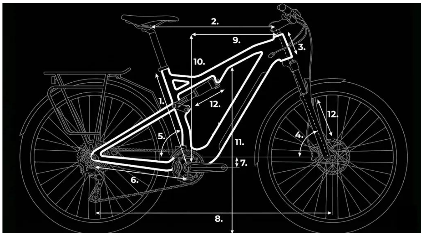
Geometria ramy Haibike ADVENTR 6 Low
