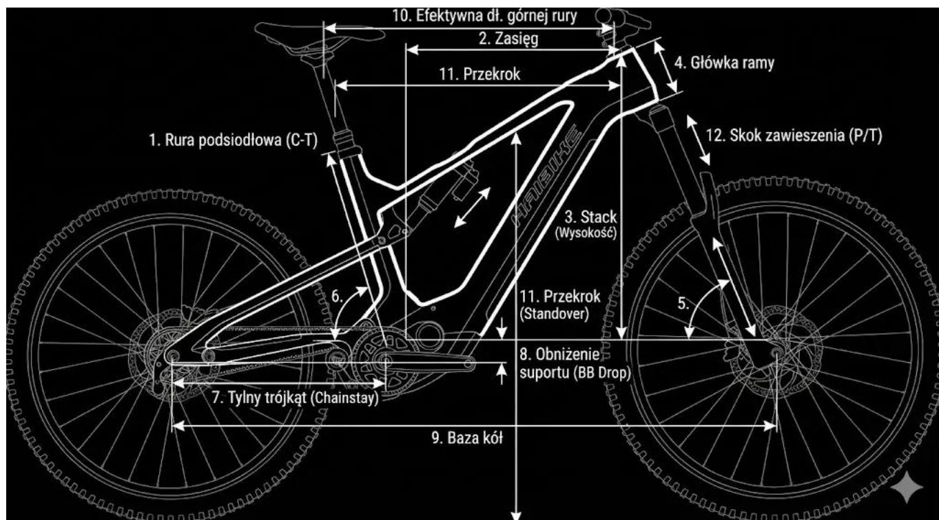
Geometria ramy Haibike LYKE CF 11
