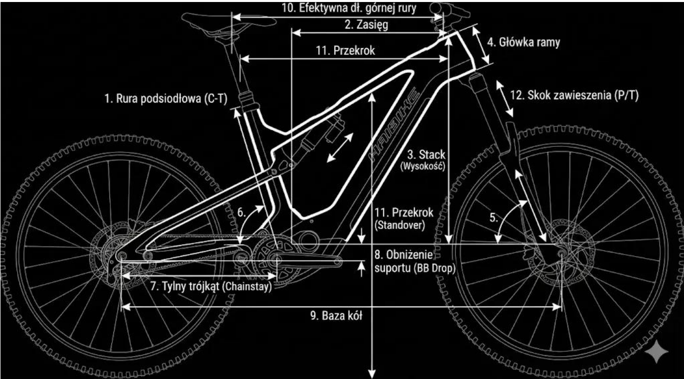
Geometria ramy Haibike HYBE CF 9
