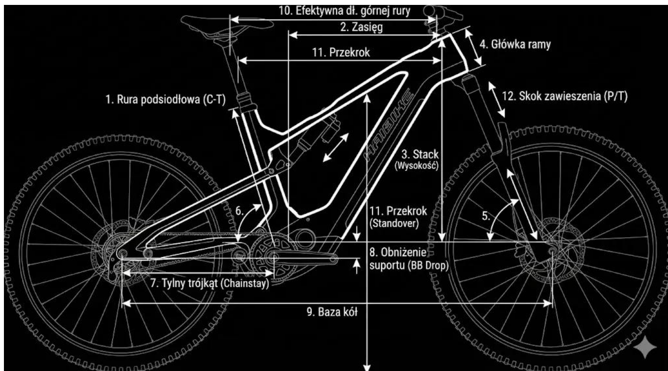
Geometria ramy Haibike HYBE CF 11
