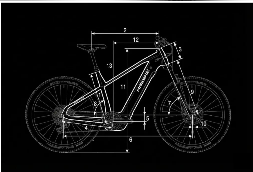
Haibike ALLTRACK 7 27.5" - Geometria Trail
