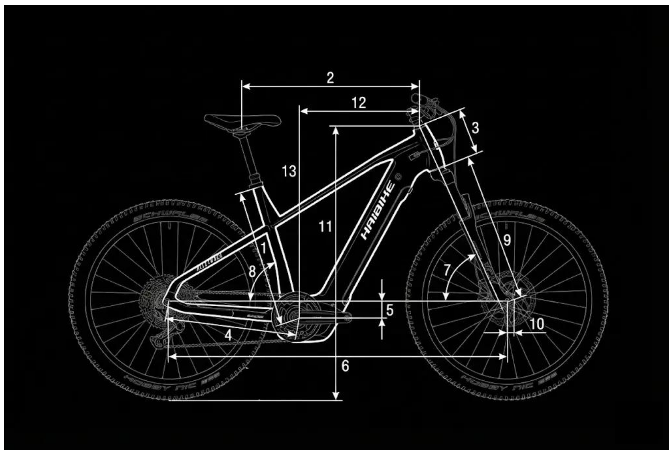
Geometria ramy Haibike ALLTRACK 11 ABS
