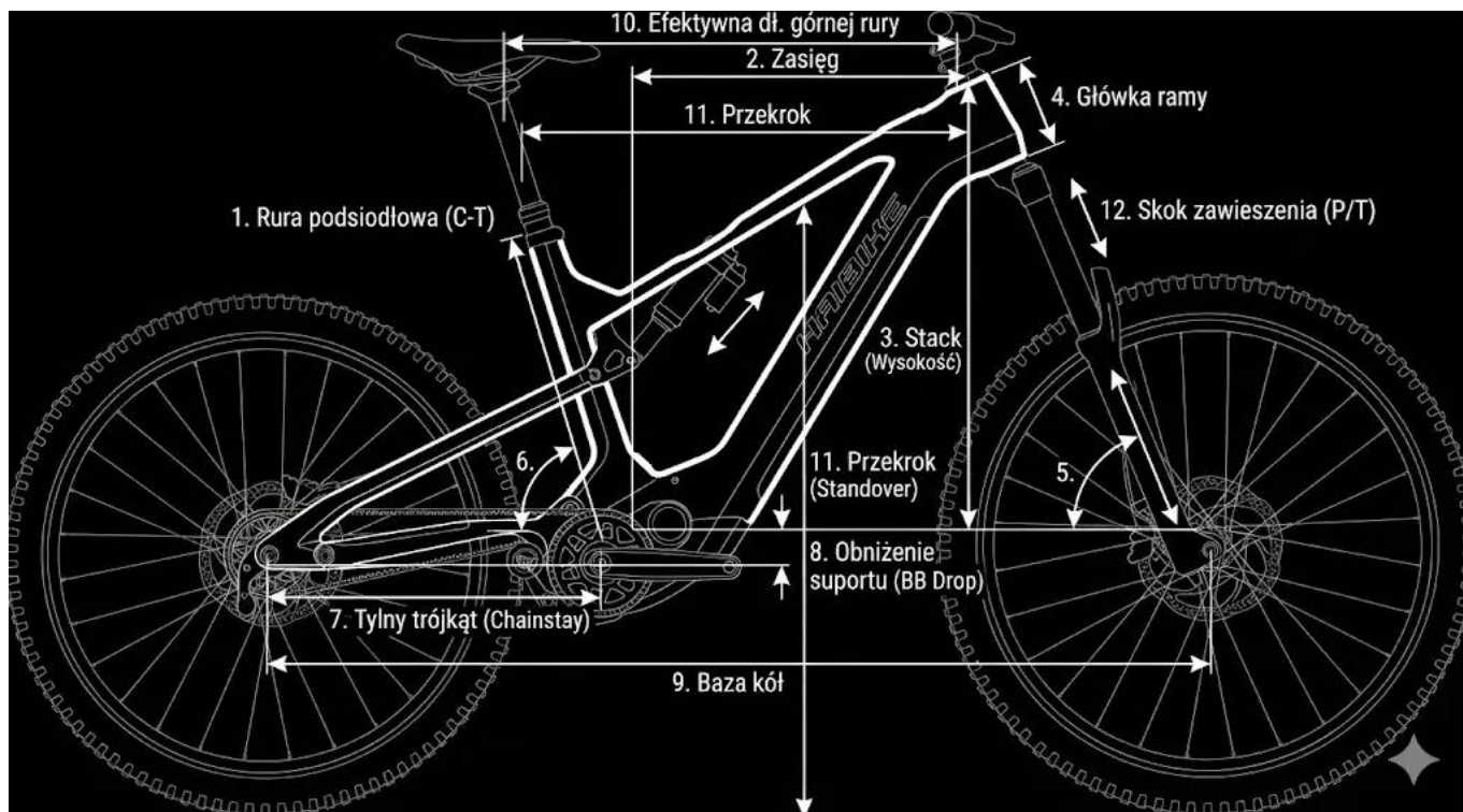
Geometria ramy Haibike ALLMTN CF 9
