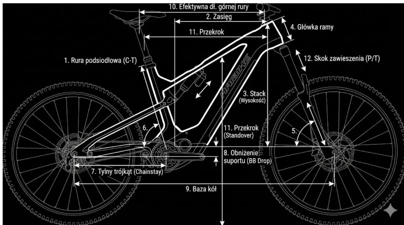
Geometria ramy Haibike ALLMTN 6
